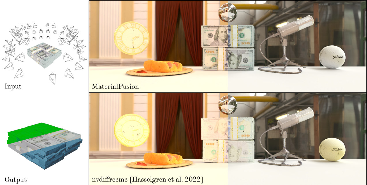
Figure 1. Given an image set of an object under unknown illumination, MaterialFusion recovers the object’s geometry, BRDF appearance, and the environmental illumination, via inverse rendering. Our method utilizes a 2D material diffusion prior to accurately reconstruct these properties. On the left, we display the input image set of the bills alongside the output of the reconstructed properties, visualized as the materials, albedo, and mesh from top to bottom, respectively. On the right, we show different objects rendered under novel lighting conditions with the reconstructed physical properties.
